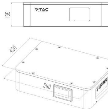
High voltage battery cluster control box
